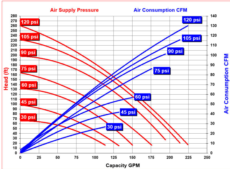
Performance Curves
